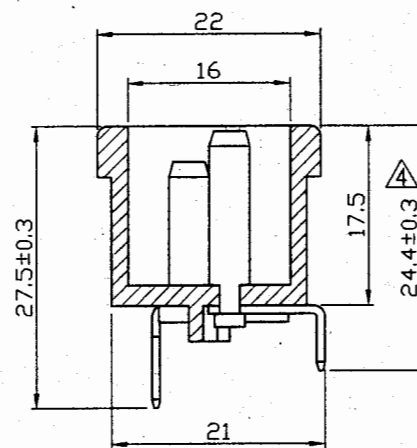
A - A SECTION
